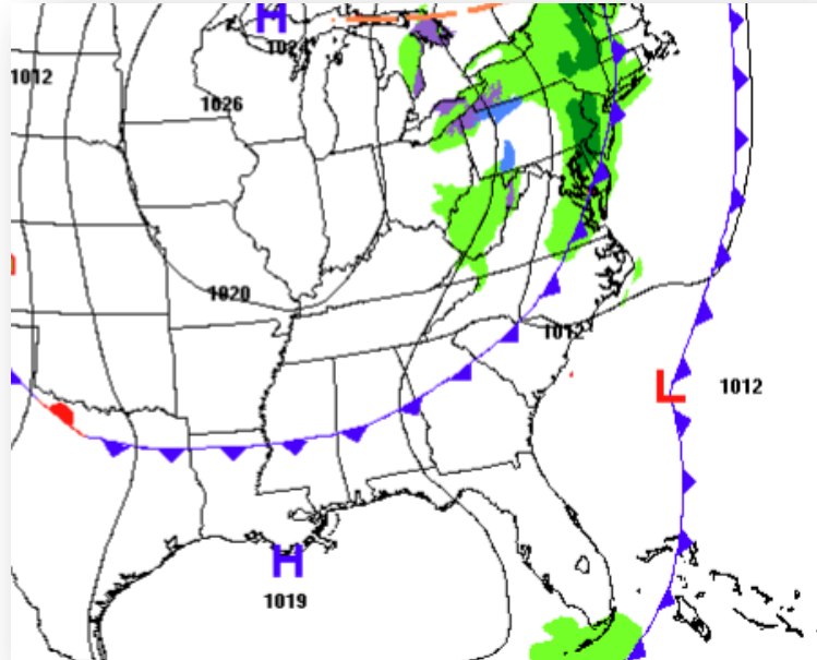
WPC – Surface Fronts/Pressure valid 7 PM Sat Apr 28, 2018
